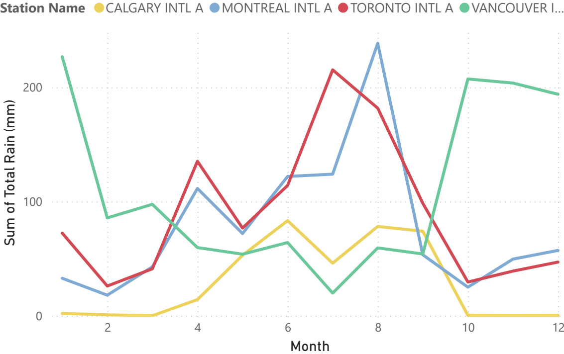
Total Rainfall (mm)
