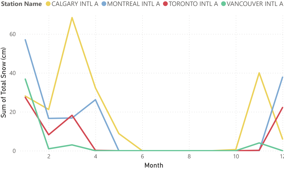
Total Snowfall (cm)
